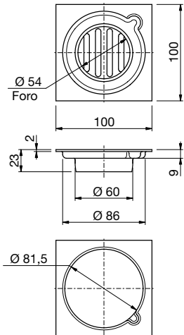
103S Attacco -Connection Ø 60mm
