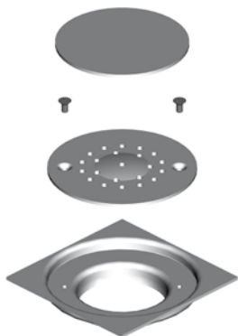
106F Floor drain with screwed grate and cover plate with central screw.
