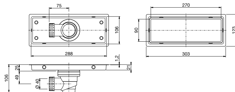
AP10030/1S LINEARDRAIN with tile holder, handmade tempered glass insert and plastic siphon
