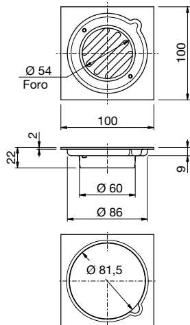
103 Attacco -Connection Ø 60mm
