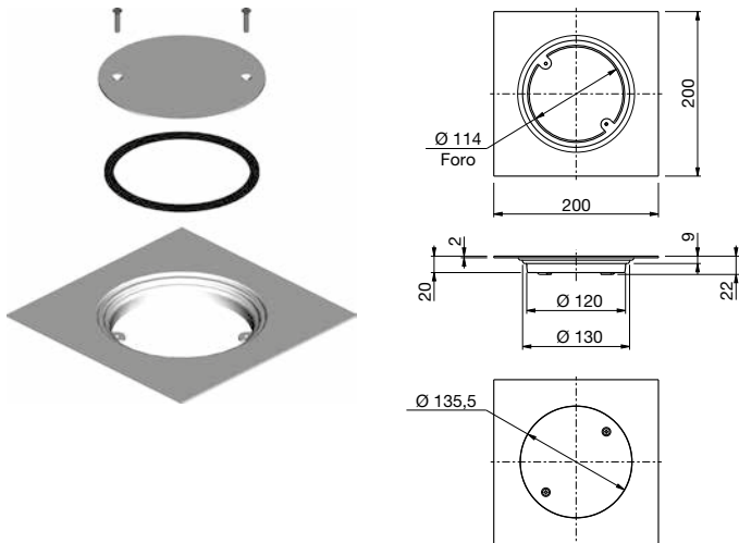
201 Cleanout with screwed cover plate and 3mm thick gasket.
