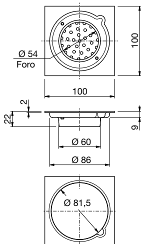
103F Attacco -Connection Ø 60mm
