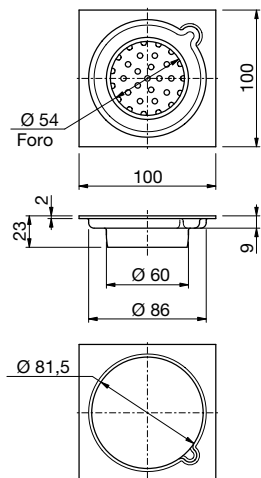
103SF Attacco -Connection Ø 60mm
