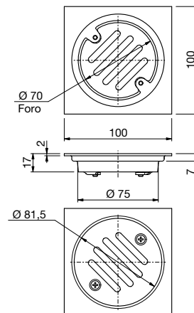
102 Attacco -Connection Ø 75mm
