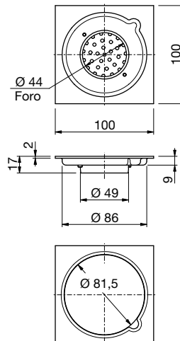
103F/49 Attacco -Connection Ø 49mm
