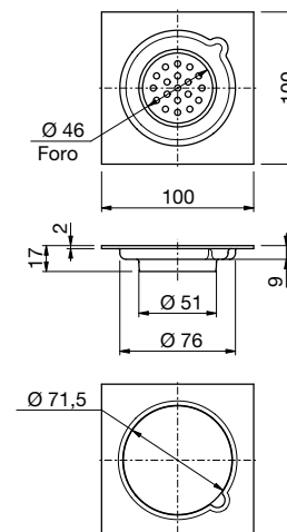
103SF/51 Attacco -Connection Ø 51mm
