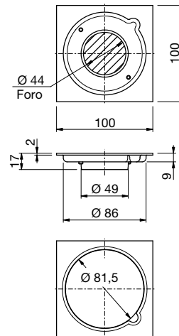
103/49 Attacco -Connection Ø 49mm
