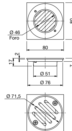
802 Floor drain with screwed grate.
