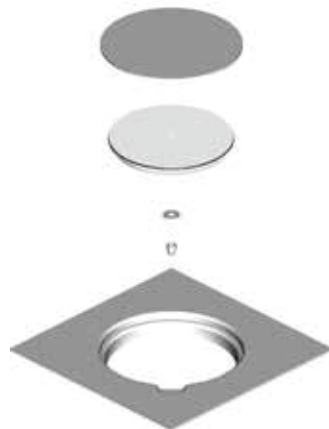
209C Floor Drain with pressure cover plate.
