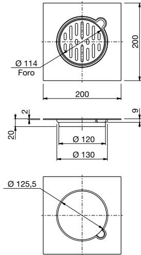
202 Floor drain with grate and cover plate.
