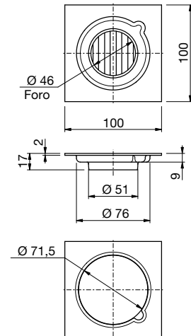
103S/51 Attacco -Connection Ø 51mm
