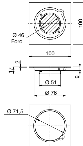
103/51 Attacco -Connection Ø 51mm
