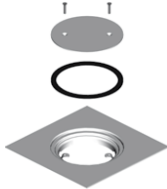
201/103 Cleanout with screwed cover plate and 3mm thick gasket.
