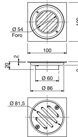
102/60 Attacco -Connection Ø 60mm
