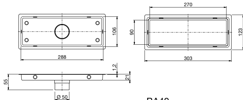
AP10030/1 LINEARDRAIN with tile holder and handmade tempered glass insert
