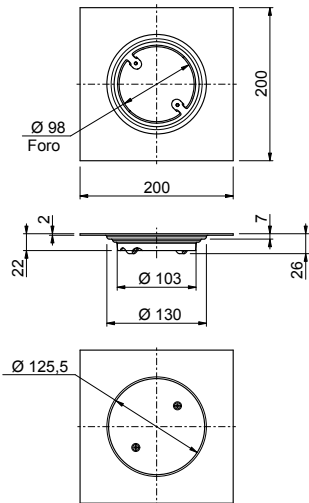
201/103 Cleanout with screwed cover plate and 3mm thick gasket.
