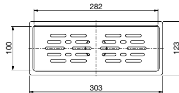
S10030 TV Con TOP VALVE®. With TOP VALVE®
