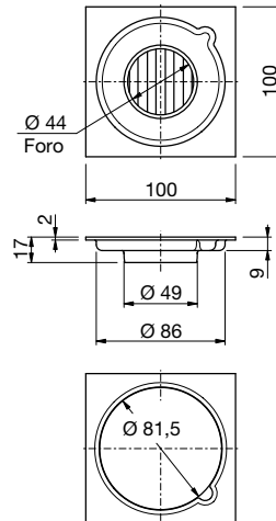
103S/49 Attacco -Connection Ø 49mm
