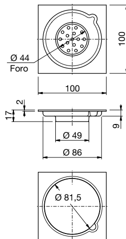
103SF/49 Attacco -Connection Ø 49mm
