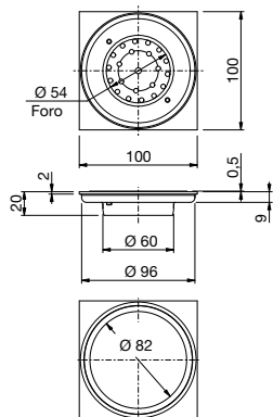
106F Floor drain with screwed grate and cover plate with central screw.
