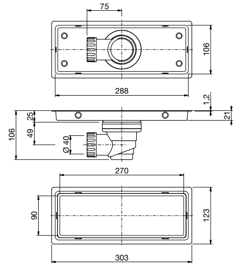
P10030/S LINEARDRAIN with tile holder and plastic siphon
