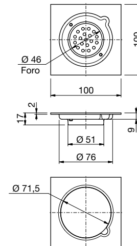
103F/51 Attacco -Connection Ø 51mm
